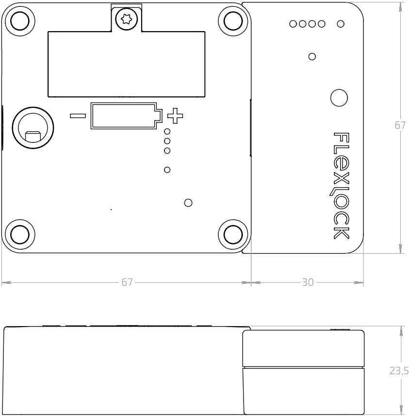
FLEXLOCK INVISIBLE WITH SMART BLUETOOTH MODULE
